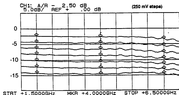
FIGURE 4. ATTENUATION vs. FREQUENCY.
