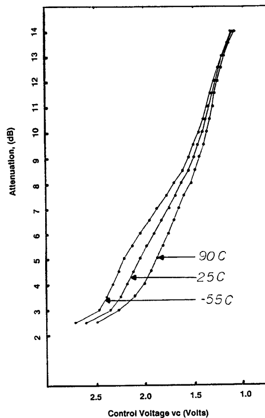
FIGURE 6. LINEAR ATTENUATOR TRANSFER CHARACTERISTICS.
